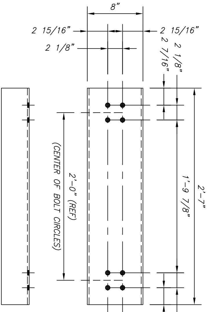
P508 DETAIL PL 1/4 X 16 X 2'-7" (BENT) WEIGHT: 35.2 # SCALE: 1/8"=1"
