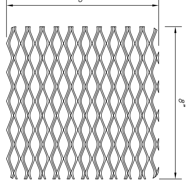
E2 DETAIL 3/4" X 9 GA X 8" EXP. METAL WEIGHT: 0.7 # SCALE: 3/8"=1"
