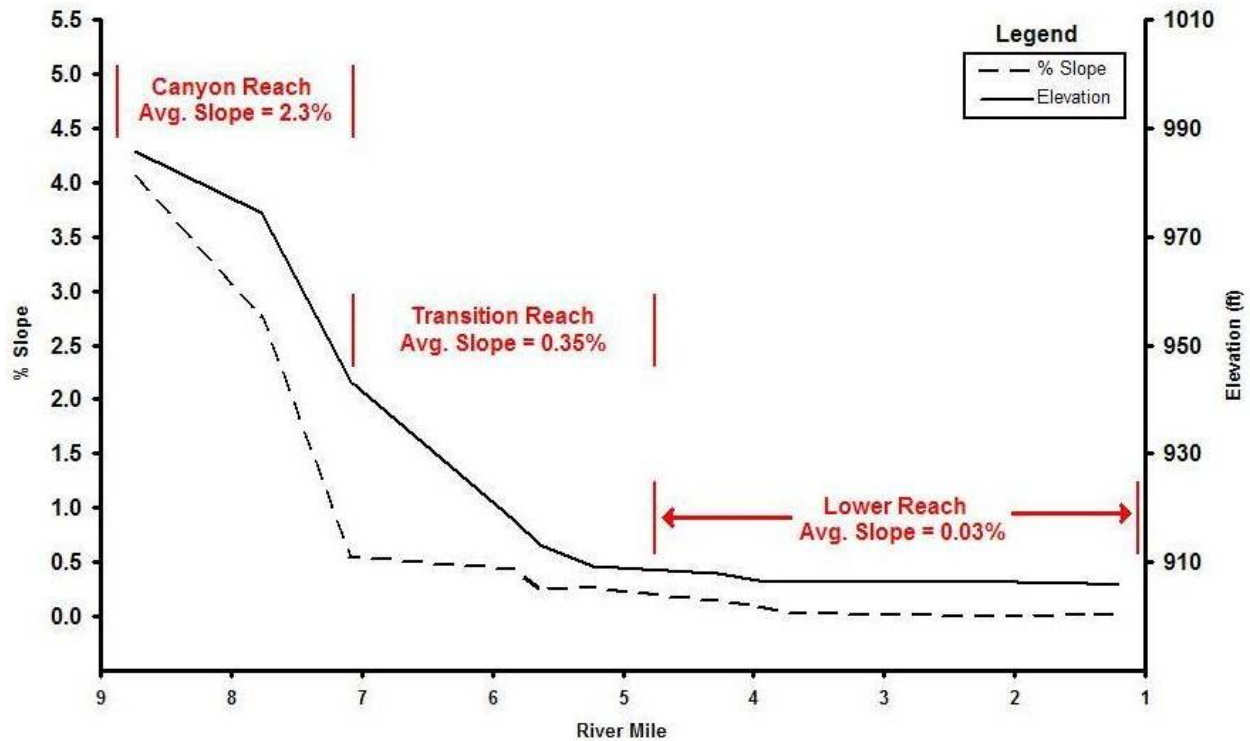
Figure 3: Chanel Gradient (defined as % slope) and Elevation of the Similkameen from the Base of Enloe Dam at RM 8.8 to the Confluence with Okanogan River at RM 0.0
